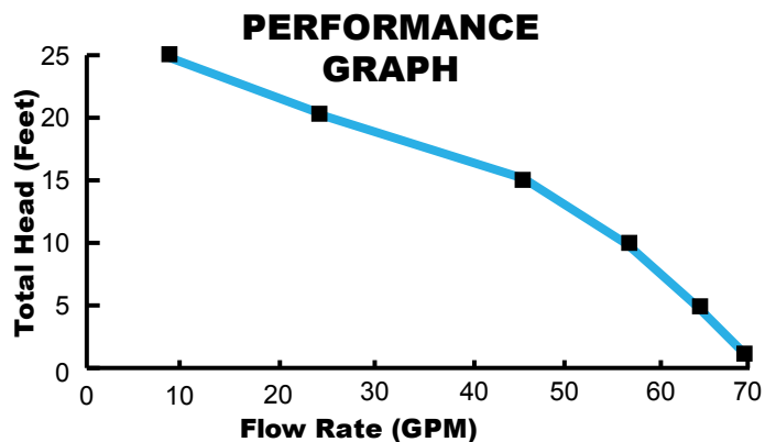
PERFORMANCE CHART
