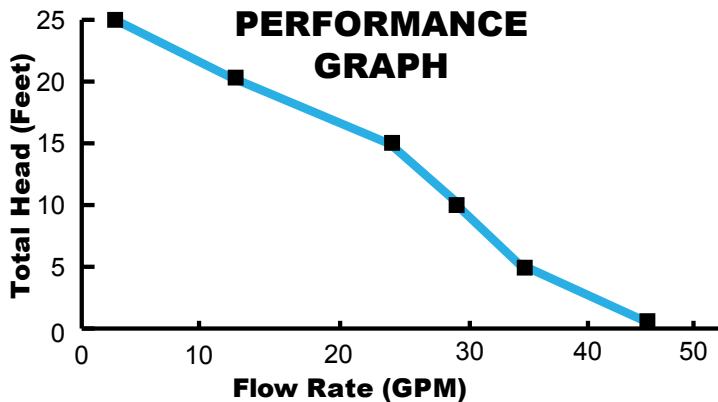
PERFORMANCE CHART
